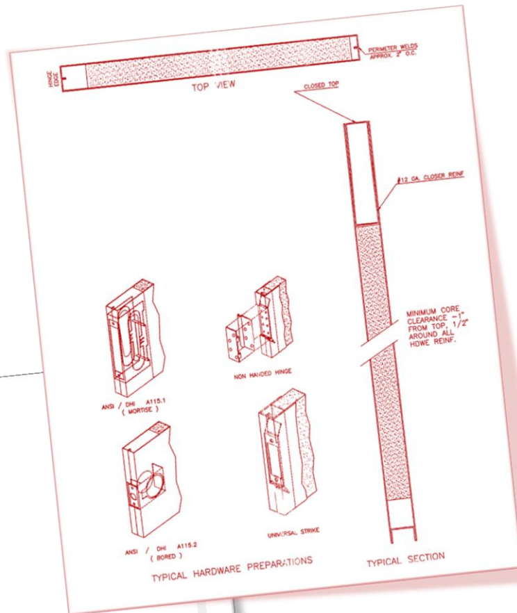
18 or 16 Gauge Galvanized Leaf with Polystyrene Core
