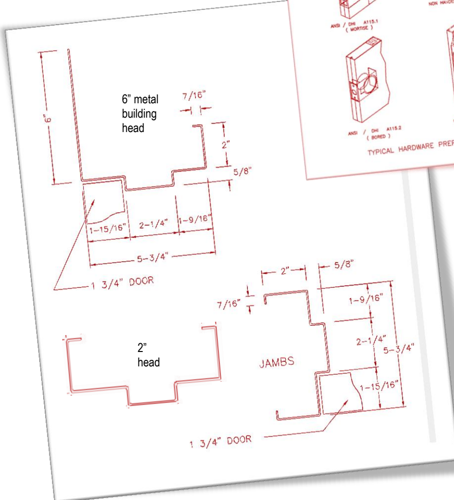
16 or 14 Gauge Galvanized 5-3/4" frame; metal building header has 6" extended face
